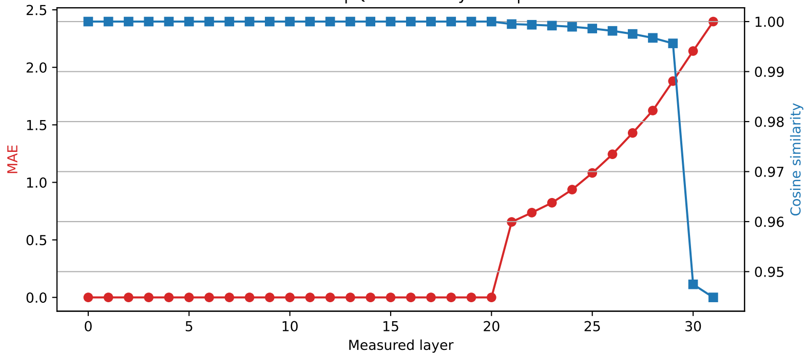
Phi-3-mini-4k-instruct | Quantized layer 20 | float64 \rightarrow int4
