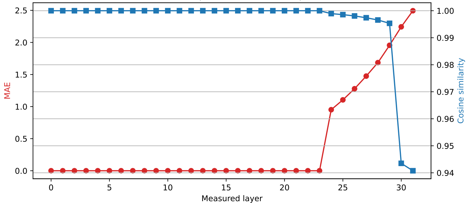
Phi-3-mini-4k-instruct | Quantized layer 23 | float64 \rightarrow int4
