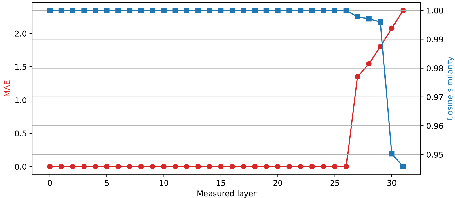
Phi-3-mini-4k-instruct | Quantized layer 26 | float64 \rightarrow int4
