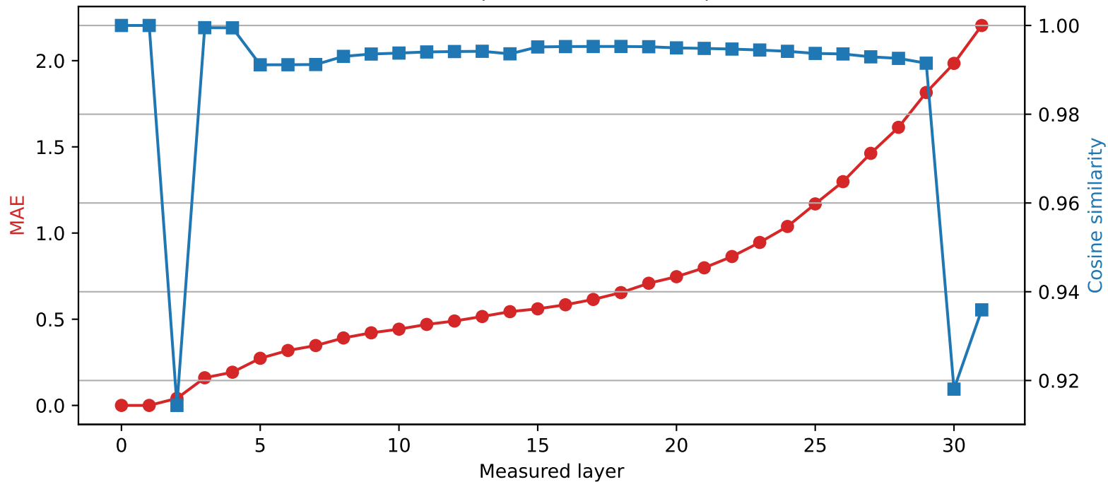
Phi-3-mini-4k-instruct | Quantized layer 1 | float64 \rightarrow int4
