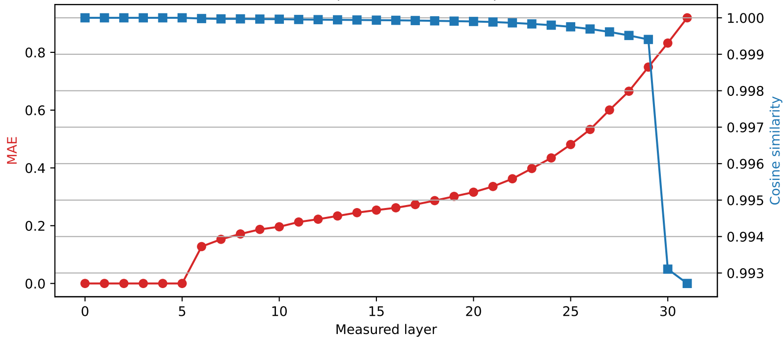
Phi-3-mini-4k-instruct | Quantized layer 5 | float64 \rightarrow int4
