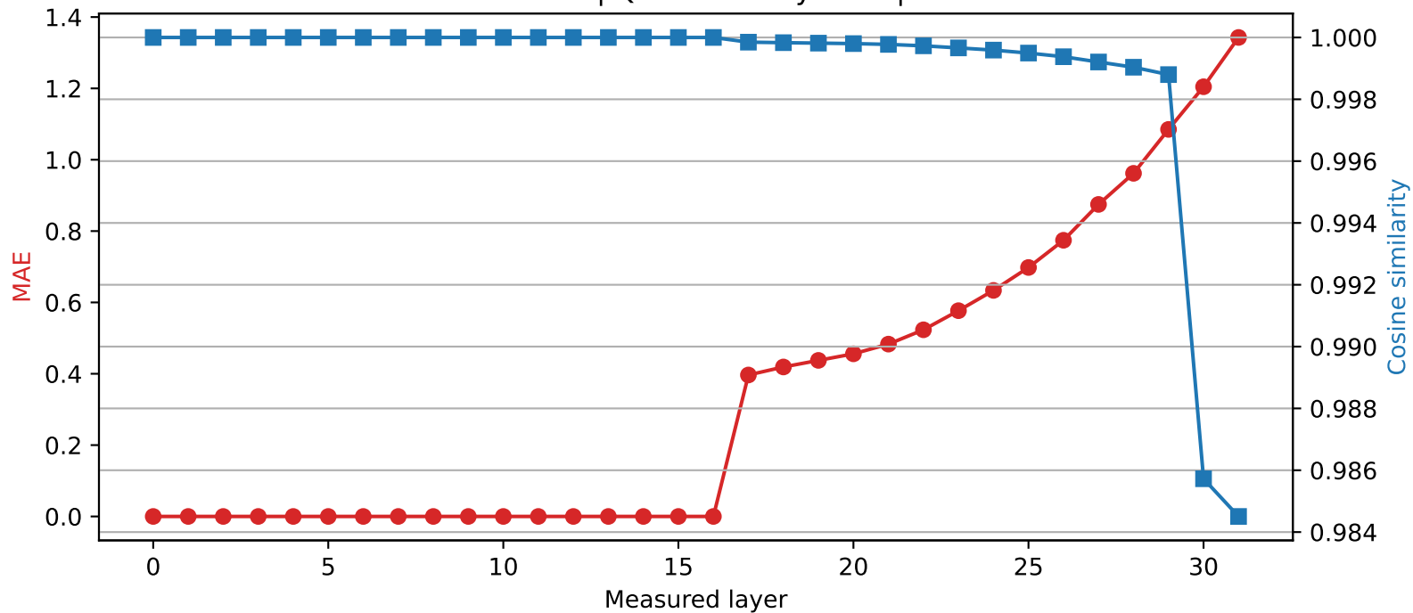
Phi-3-mini-4k-instruct | Quantized layer 16 | float64 \rightarrow int4
