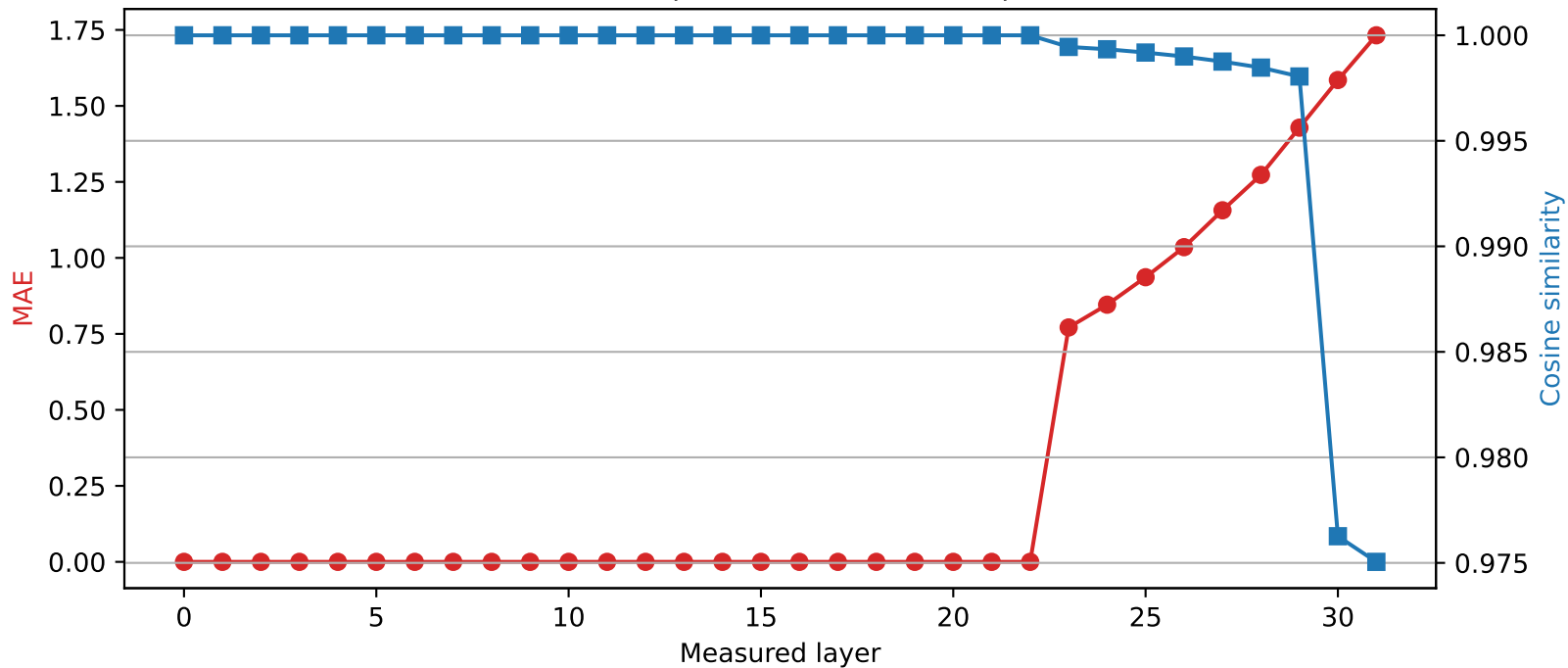
Phi-3-mini-4k-instruct | Quantized layer 22 | float64 \rightarrow int4
