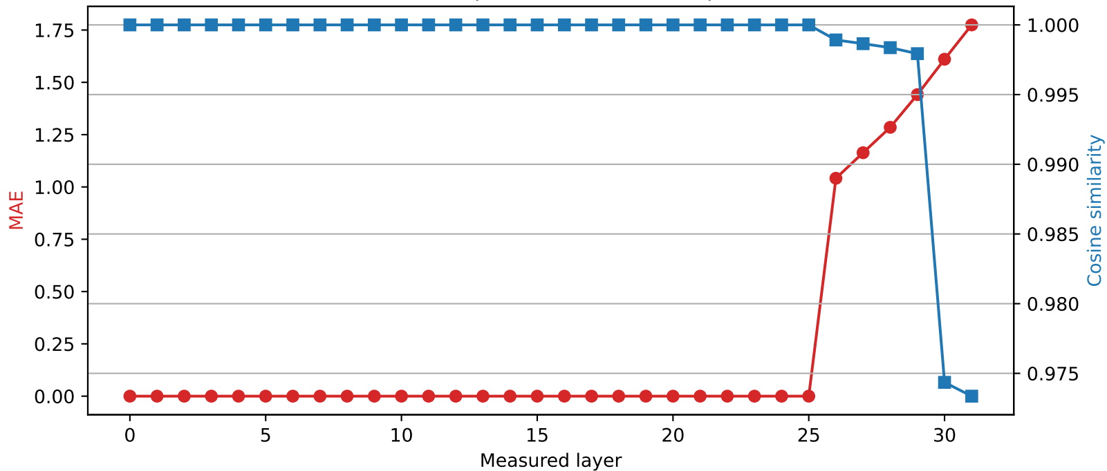
Phi-3-mini-4k-instruct | Quantized layer 25 | float64 \rightarrow int4
