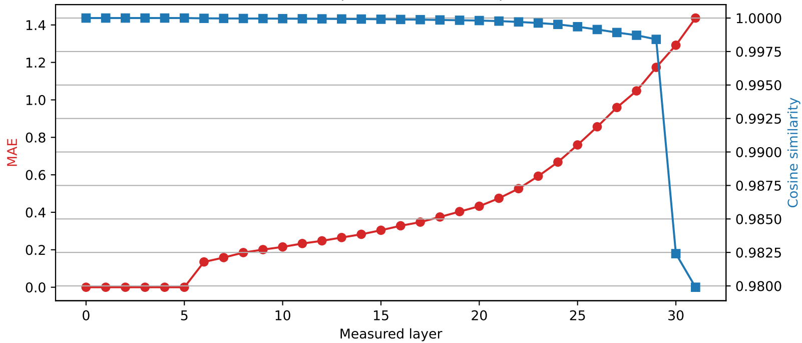
Phi-3-mini-4k-instruct | Quantized layer 5 | float64 → int4
