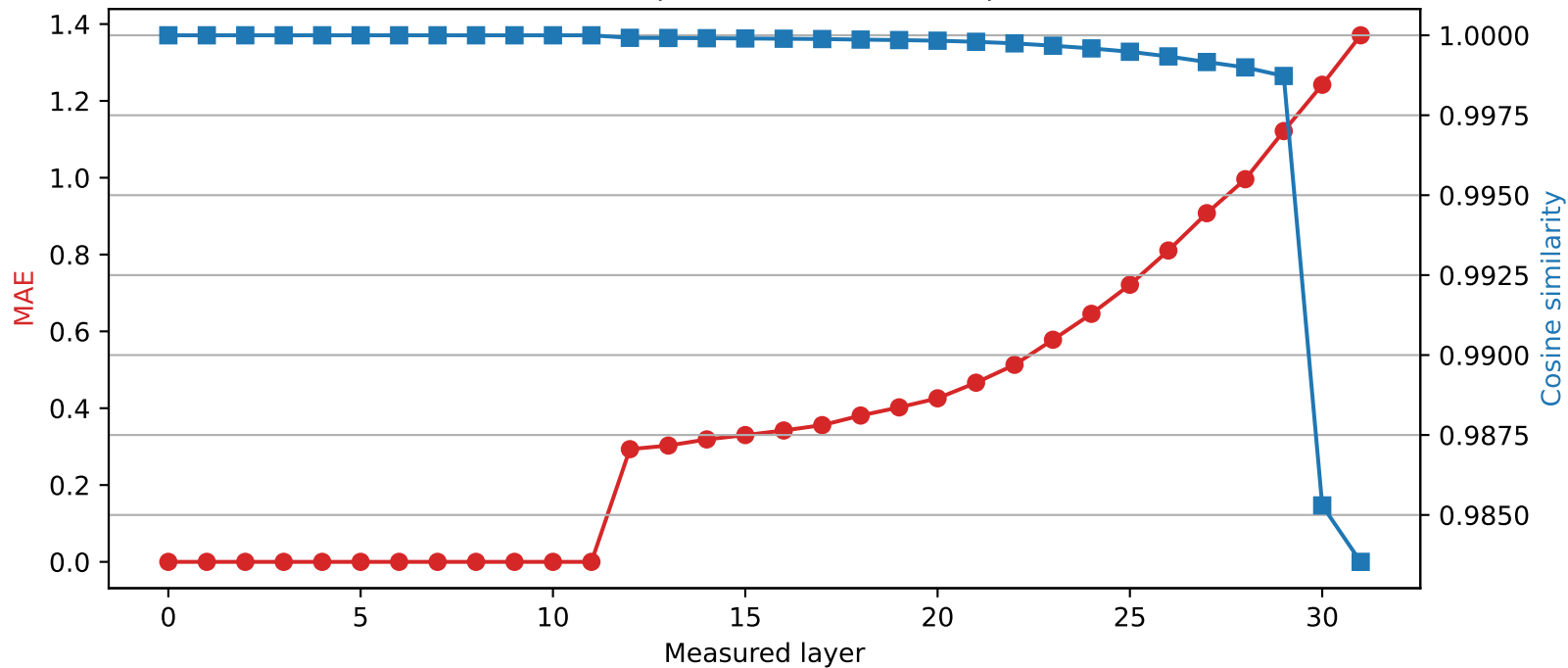
Phi-3-mini-4k-instruct | Quantized layer 11 | float64 \rightarrow int4
