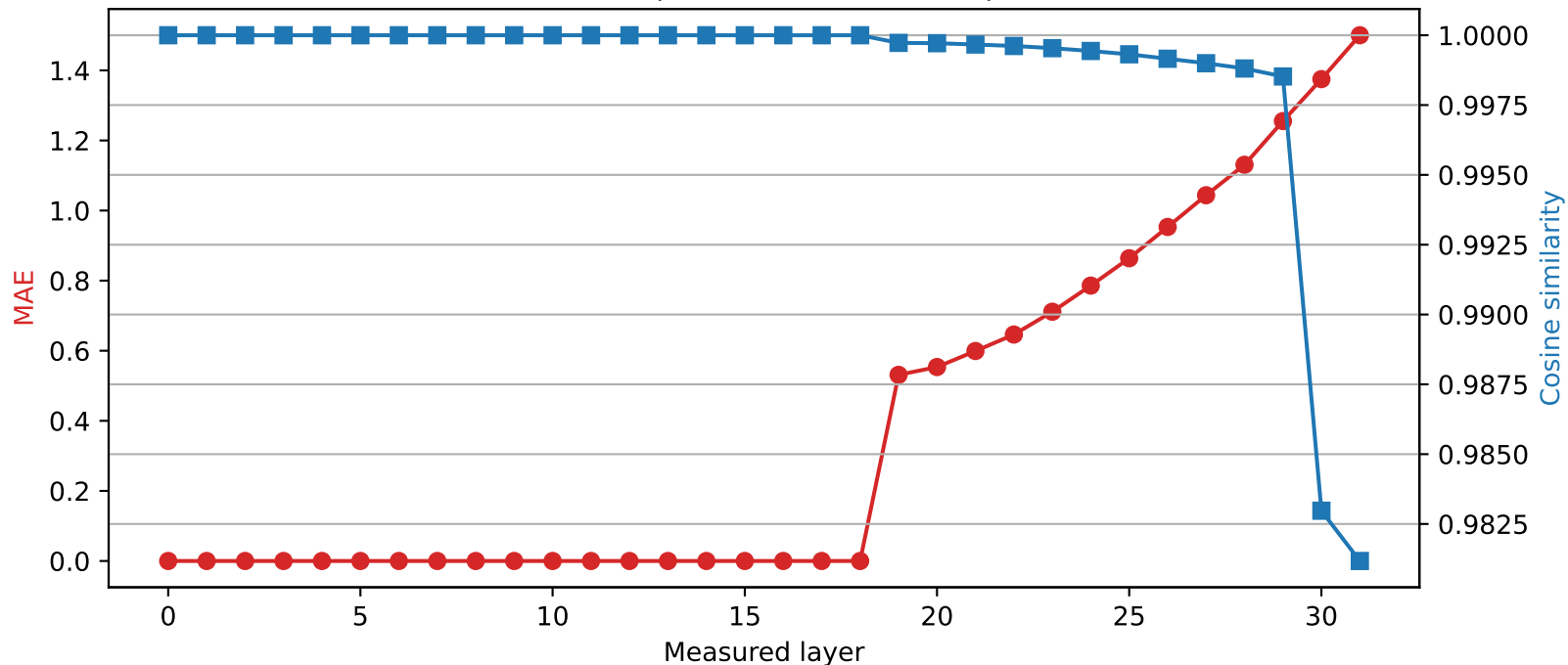
Phi-3-mini-4k-instruct | Quantized layer 18 | float64 \rightarrow int4
