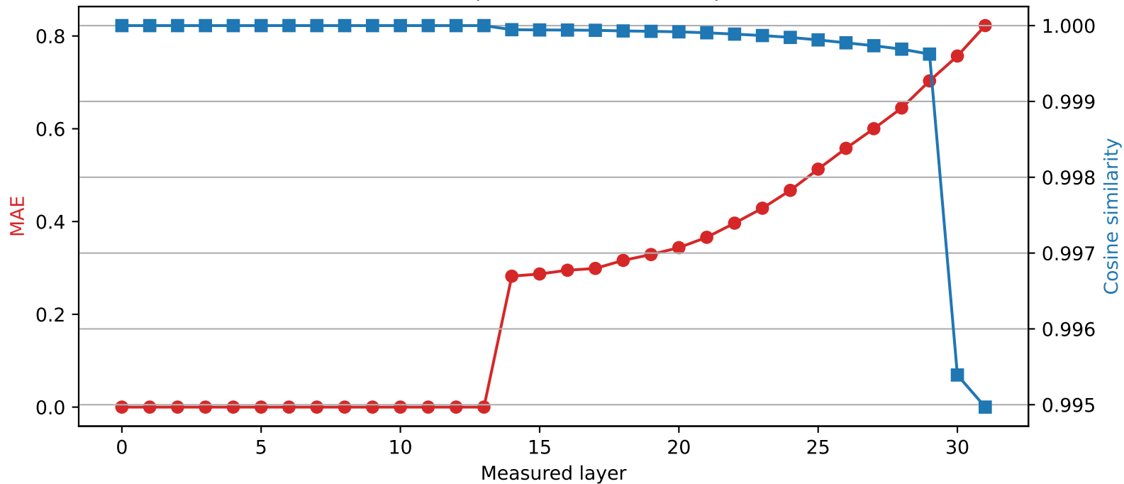
Phi-3-mini-4k-instruct | Quantized layer 13 | float64 \rightarrow int4
