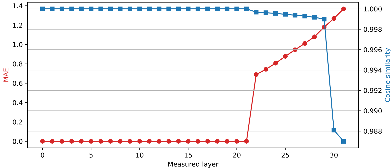
Phi-3-mini-4k-instruct | Quantized layer 21 | float64 \rightarrow int4
