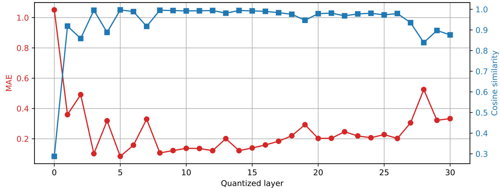
Phi-3-mini-4k-instruct | Prompt 0 Final RMSNorm output damage | float64 \rightarrow int2
