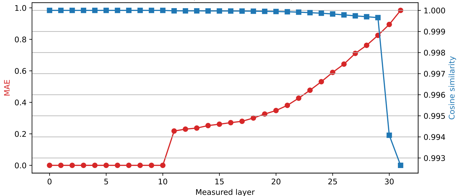
Phi-3-mini-4k-instruct | Quantized layer 10 | float64 → int2
