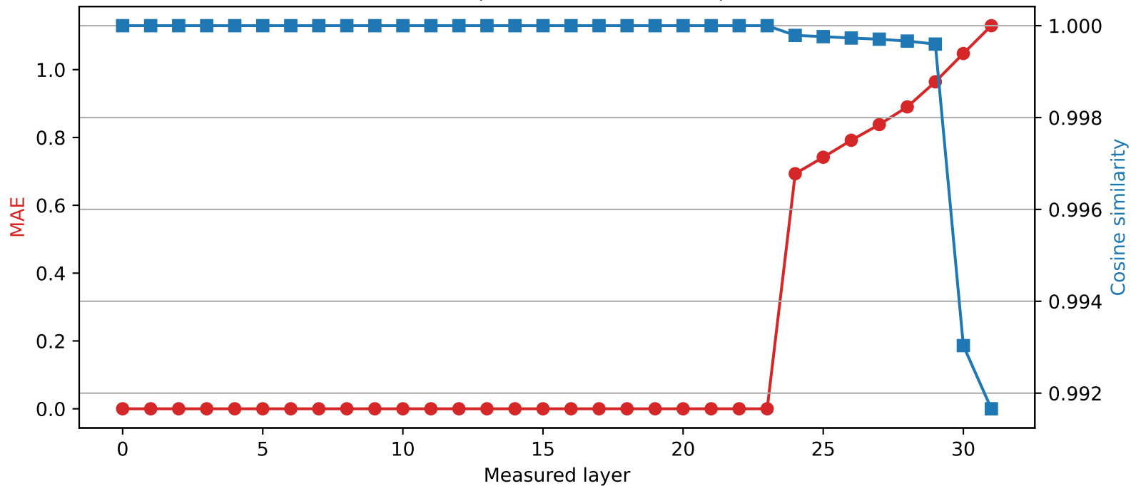
Phi-3-mini-4k-instruct | Quantized layer 23 | float64 → int2
