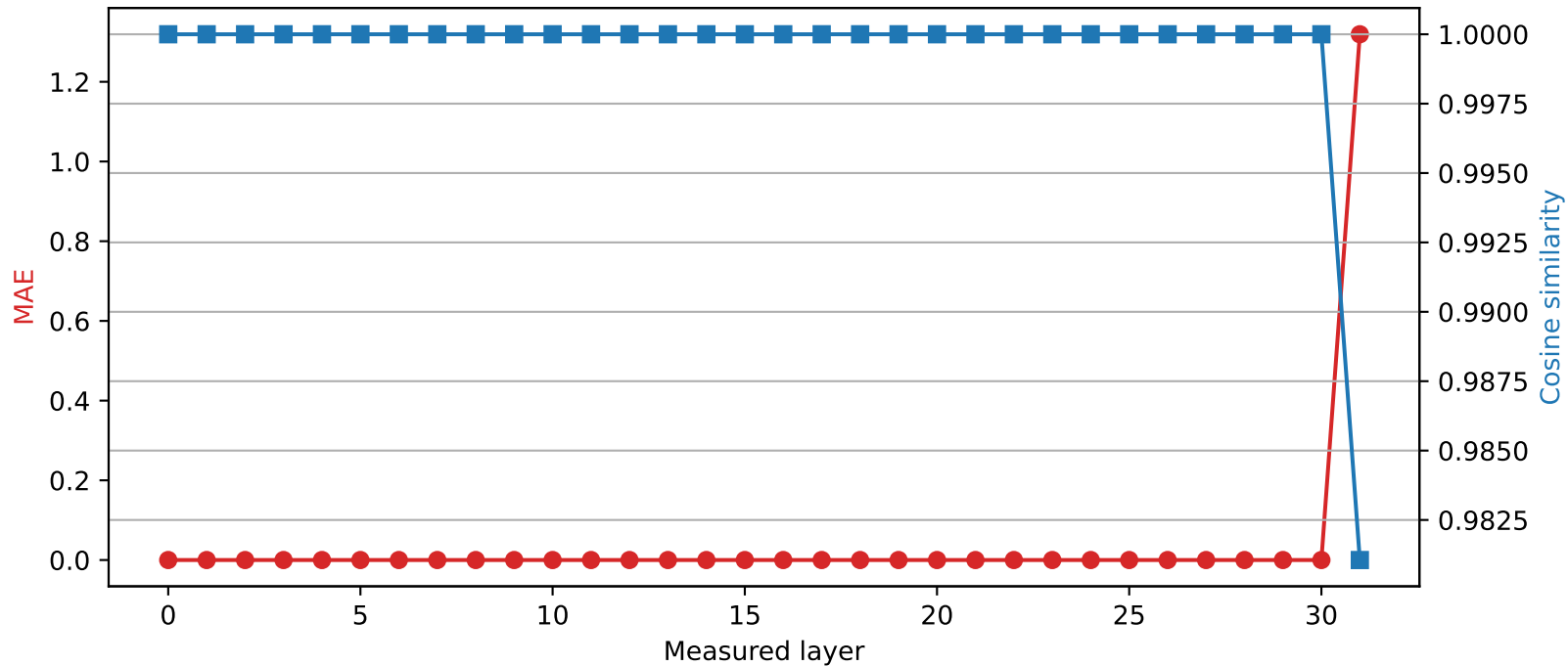
Phi-3-mini-4k-instruct | Quantized layer 30 | float64 → int2
