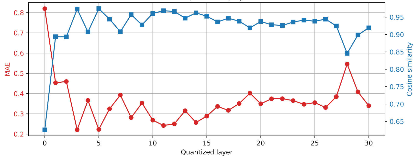
Phi-3-mini-4k-instruct | Prompt 1 Final RMSNorm output damage | float64 \rightarrow int2
