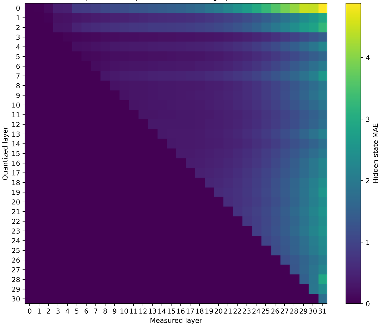
Phi-3-mini-4k-instruct Prompt 1: MAE representation damage | float64 \rightarrow int2
