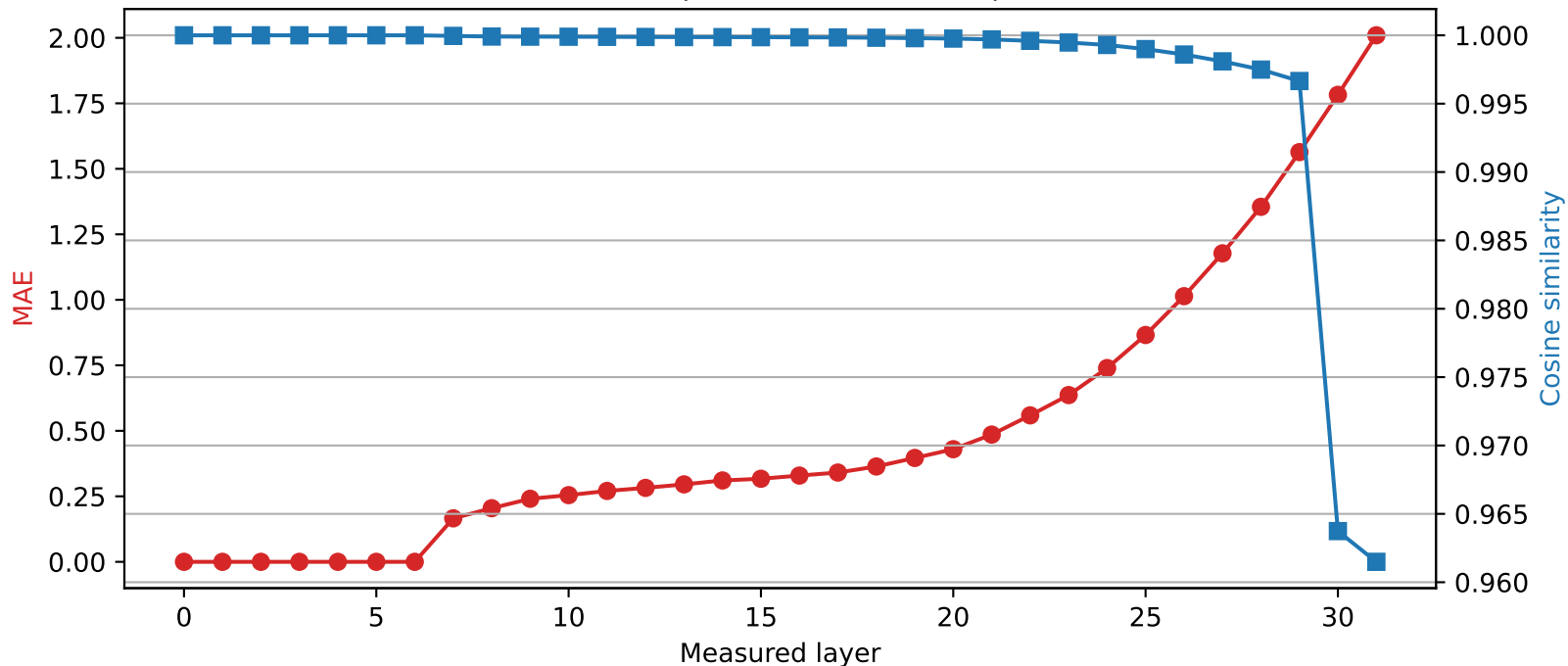
Phi-3-mini-4k-instruct | Quantized layer 6 | float64 \rightarrow int2
