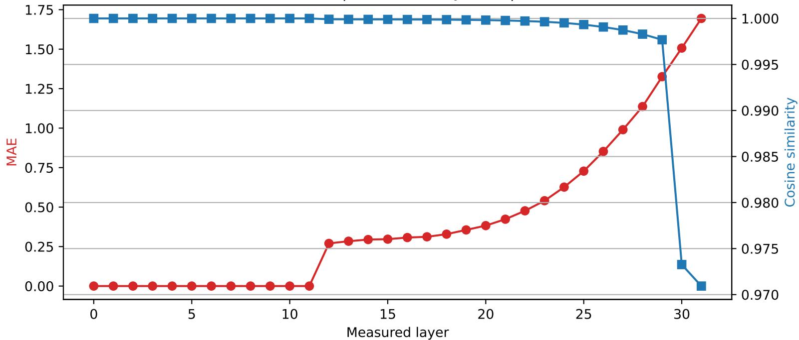
Phi-3-mini-4k-instruct | Quantized layer 11 | float64 \rightarrow int2
