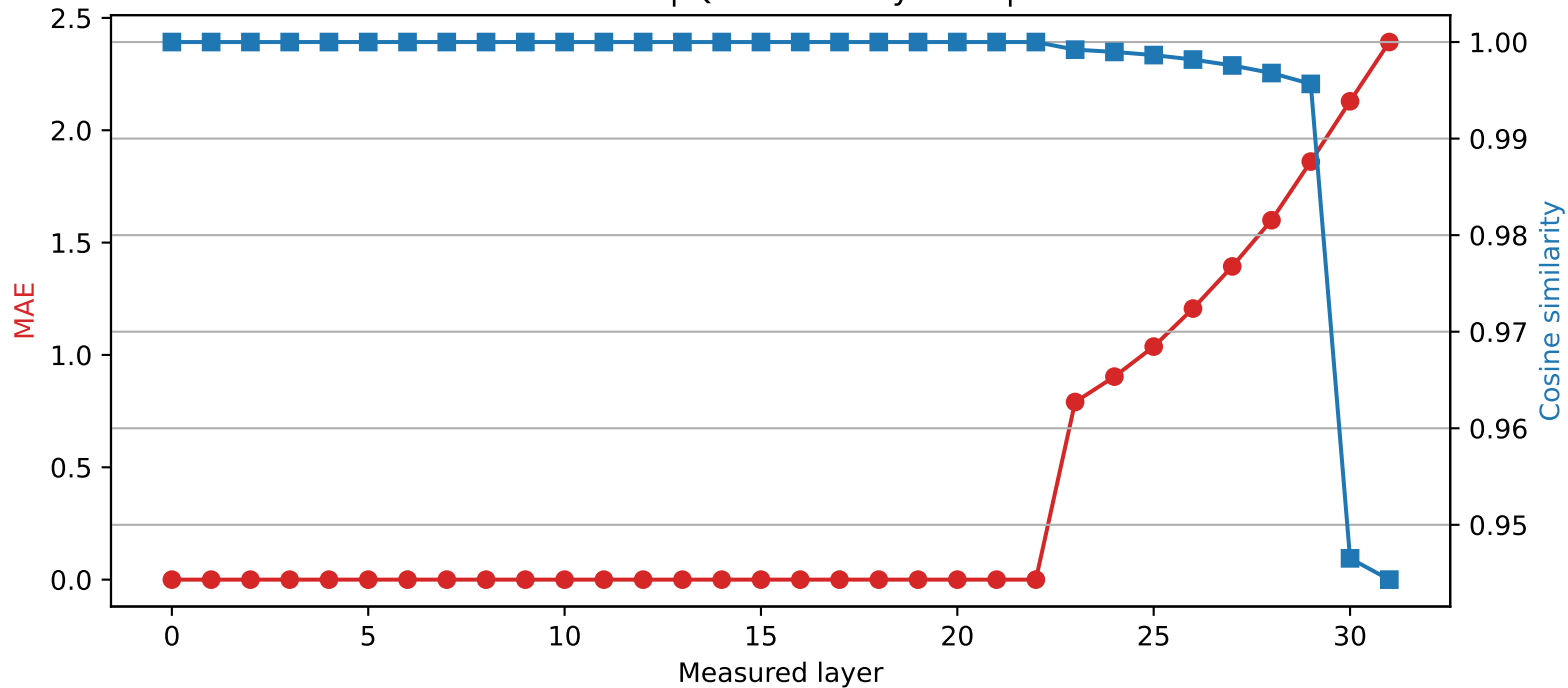
Phi-3-mini-4k-instruct | Quantized layer 22 | float64 \rightarrow int2
