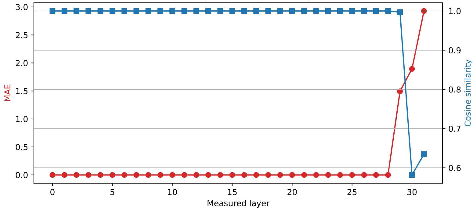
Phi-3-mini-4k-instruct | Quantized layer 28 | float64 → int2
