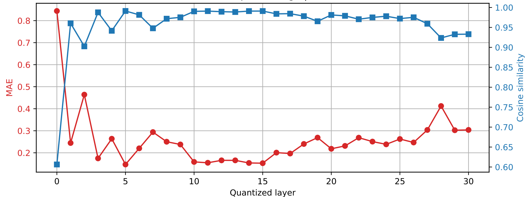
Phi-3-mini-4k-instruct | Prompt 2 Final RMSNorm output damage | float64 \rightarrow int2
