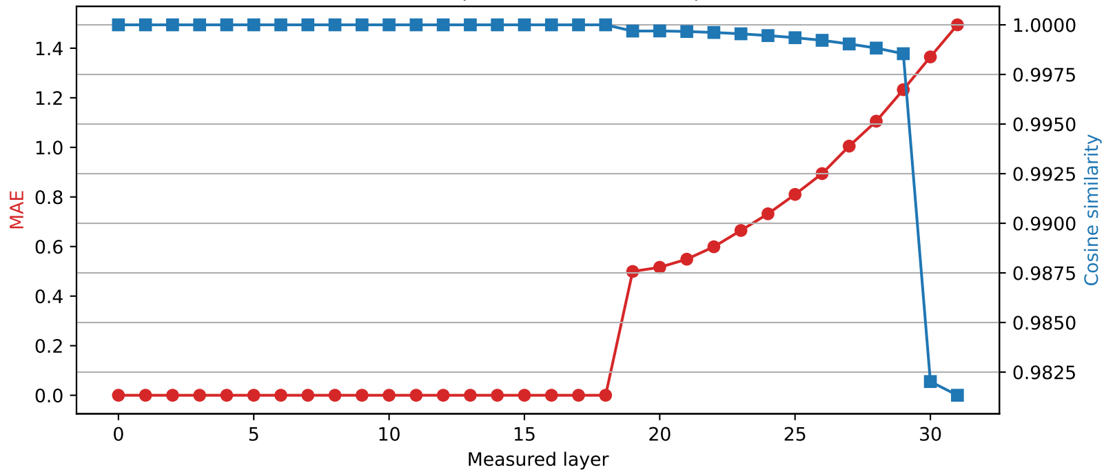
Phi-3-mini-4k-instruct | Quantized layer 18 | float64 → int2
