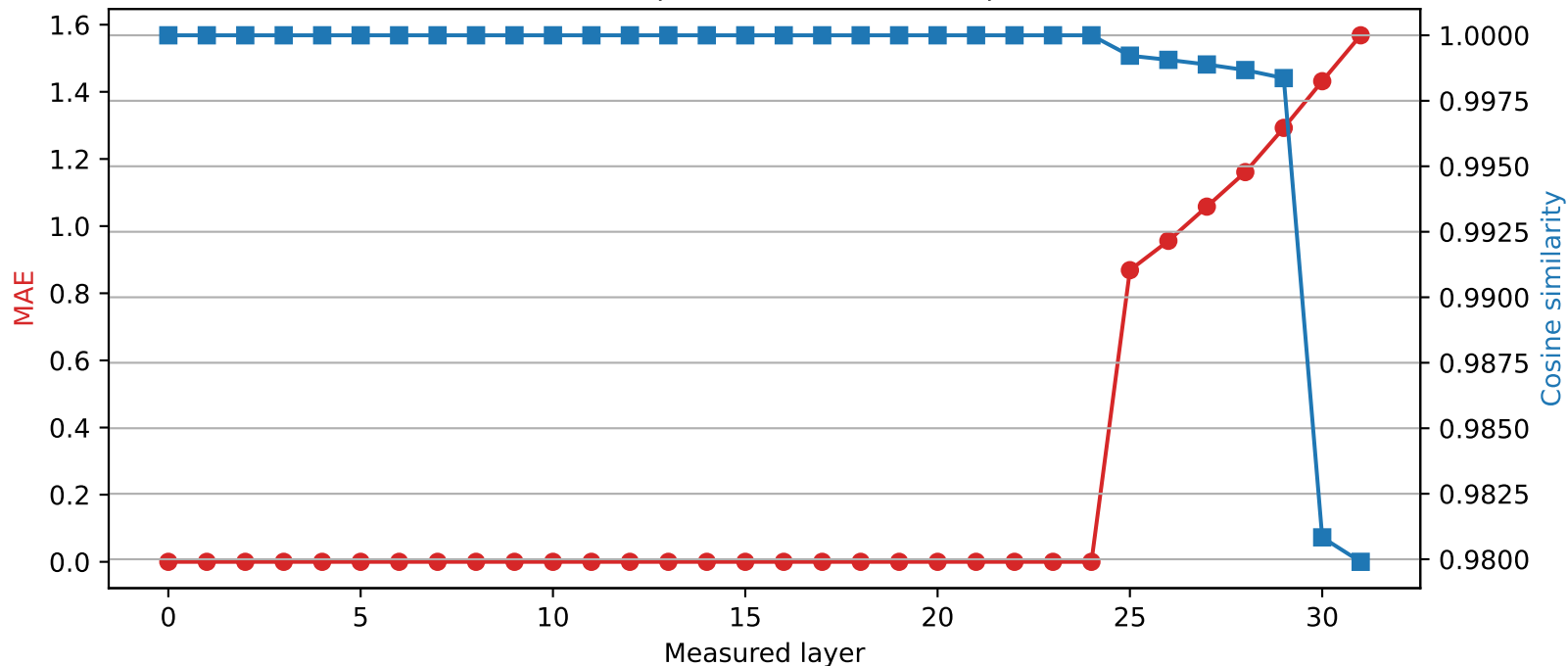
Phi-3-mini-4k-instruct | Quantized layer 24 | float64 \rightarrow int2
