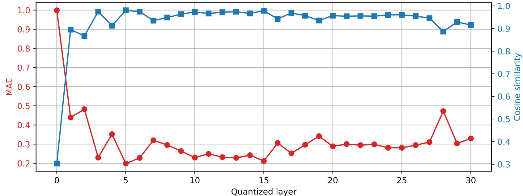
Phi-3-mini-4k-instruct | Prompt 3 Final RMSNorm output damage | float64 \rightarrow int2
