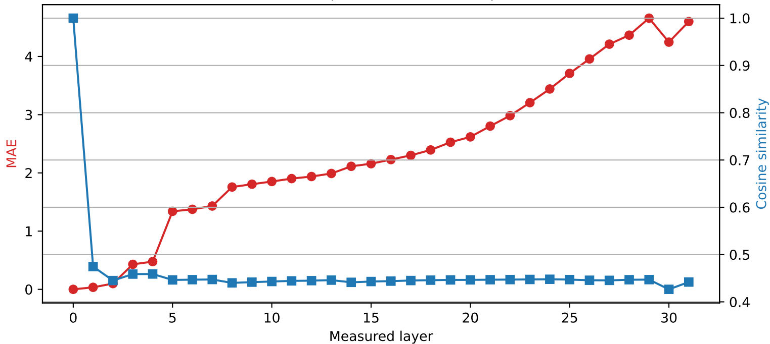
Phi-3-mini-4k-instruct | Quantized layer 0 | float64 \rightarrow int2
