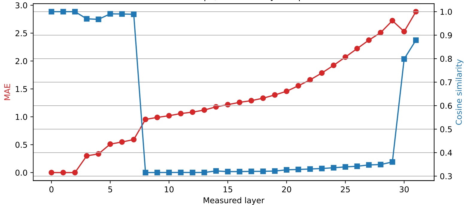
Phi-3-mini-4k-instruct | Quantized layer 2 | float64 → int2
