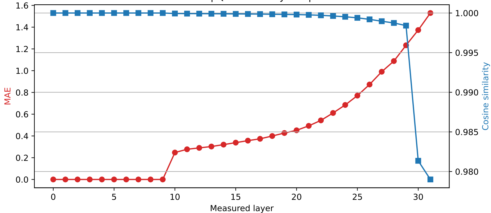
Phi-3-mini-4k-instruct | Quantized layer 9 | float64 \rightarrow int2
