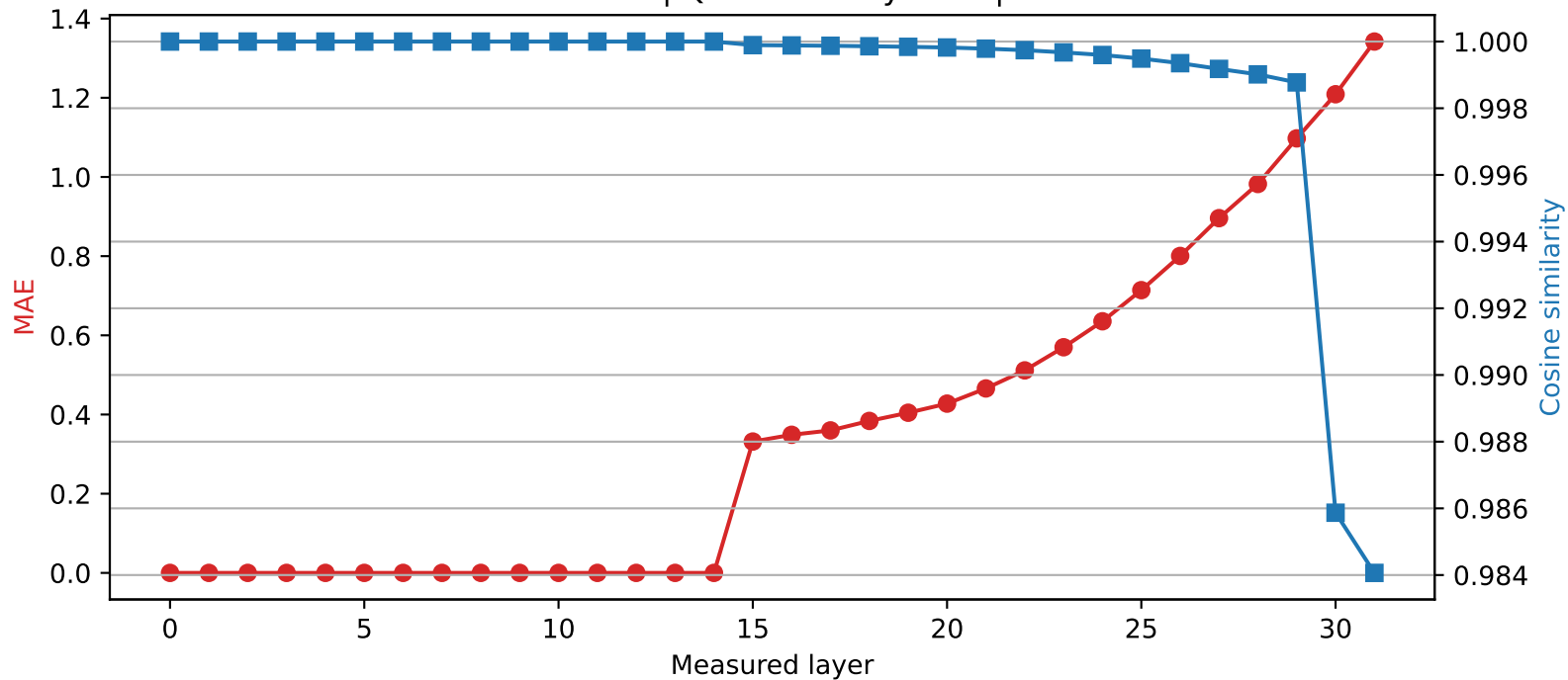
Phi-3-mini-4k-instruct | Quantized layer 14 | float64 \rightarrow int2
