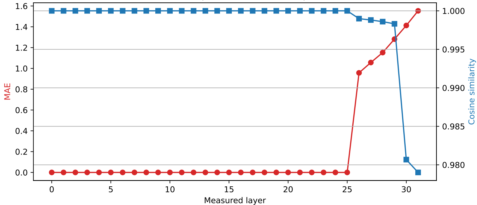
Phi-3-mini-4k-instruct | Quantized layer 25 | float64 \rightarrow int2
