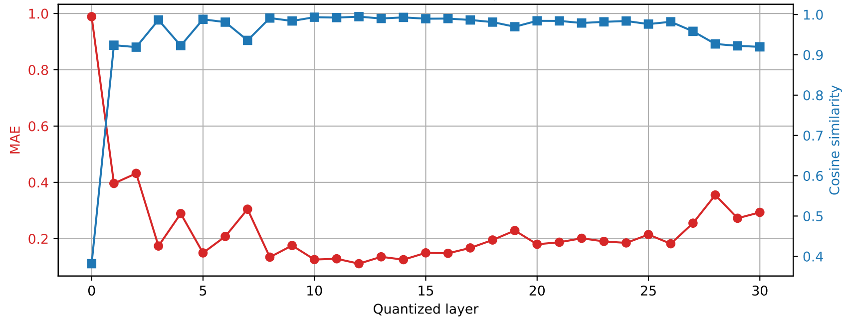
Phi-3-mini-4k-instruct | Prompt 4 Final RMSNorm output damage | float64 \rightarrow int2
