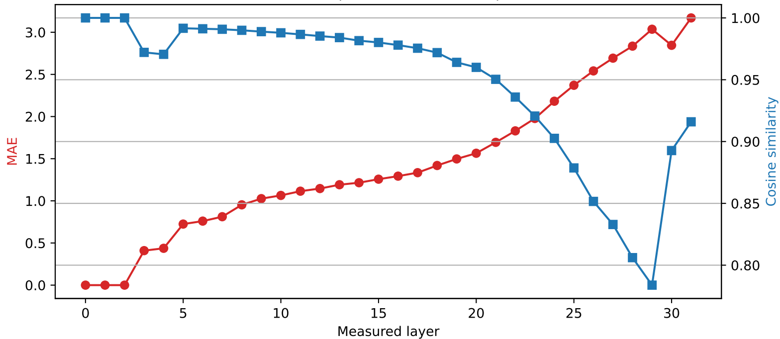
Phi-3-mini-4k-instruct | Quantized layer 2 | float64 \rightarrow int2
