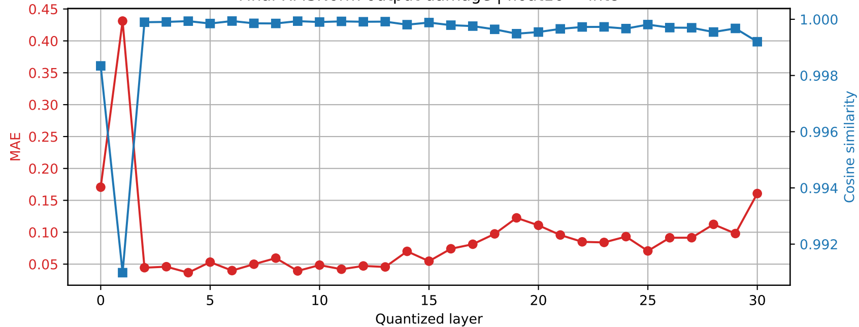
Mistral-7B-Instruct-v0.3 | Prompt 0 Final RMSNorm output damage | float16 \rightarrow int8
