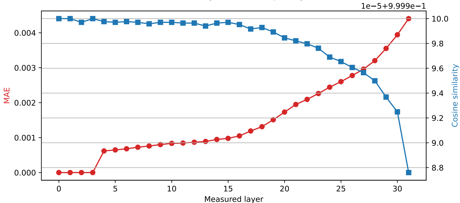
Mistral-7B-Instruct-v0.3 | Quantized layer 3 | float16 → int8
