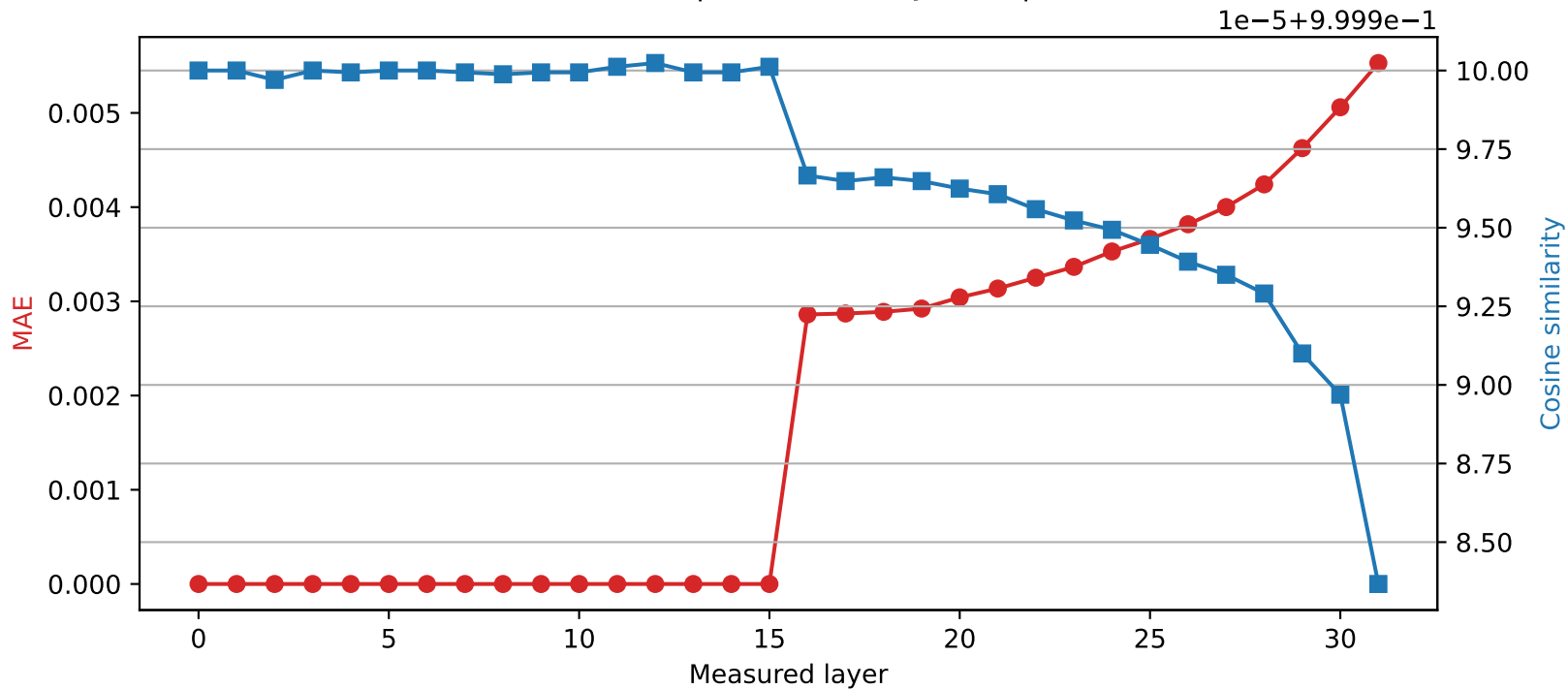
Mistral-7B-Instruct-v0.3 | Quantized layer 15 | float16 \rightarrow int8
