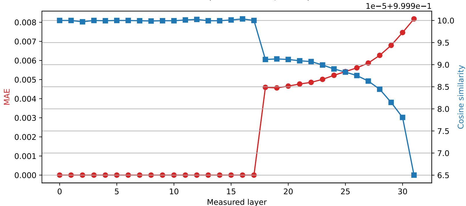
Mistral-7B-Instruct-v0.3 | Quantized layer 17 | float16 → int8
