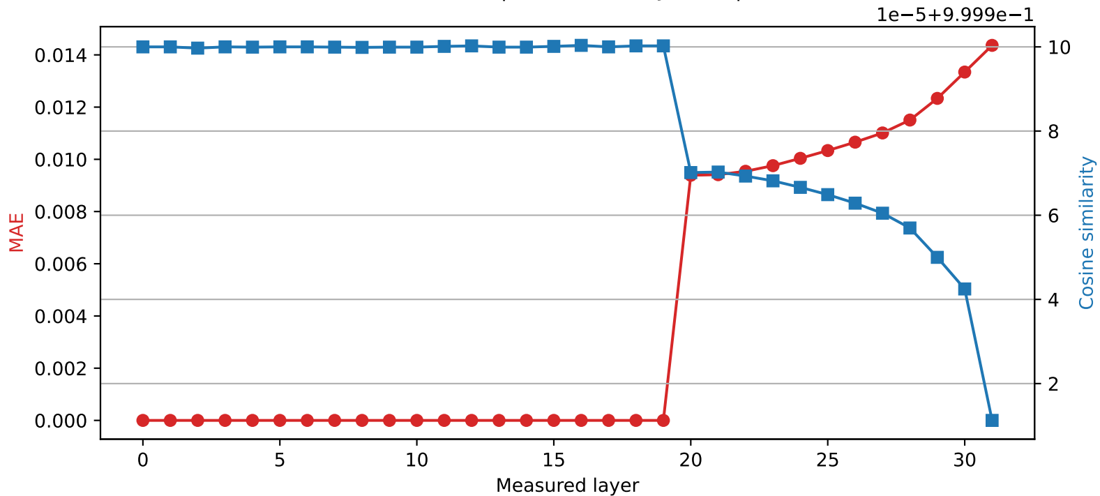
Mistral-7B-Instruct-v0.3 | Quantized layer 19 | float16 → int8
