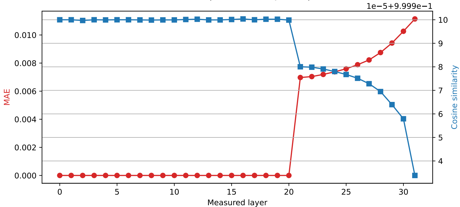
Mistral-7B-Instruct-v0.3 | Quantized layer 20 | float16 \rightarrow int8
