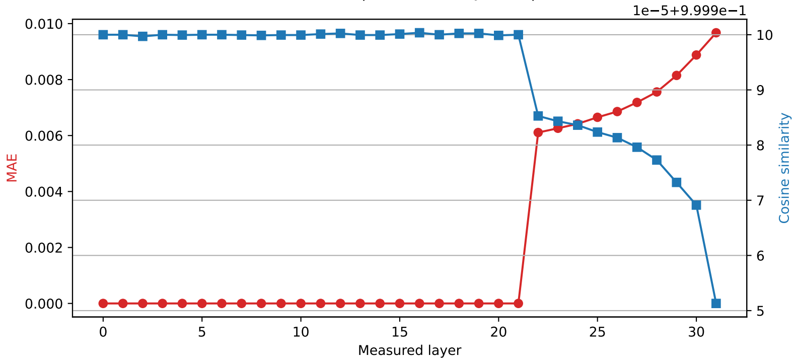
Mistral-7B-Instruct-v0.3 | Quantized layer 21 | float16 → int8
