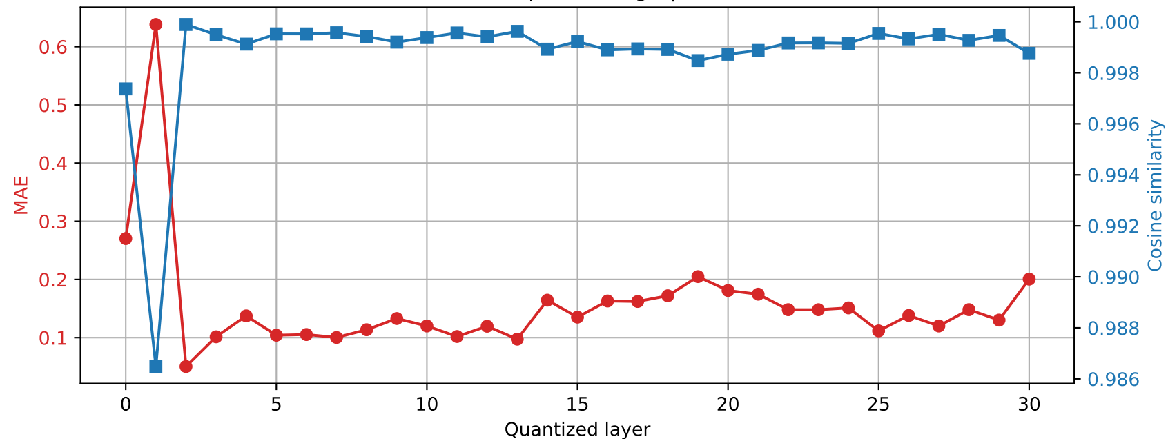
Mistral-7B-Instruct-v0.3 | Prompt 1 Final RMSNorm output damage | float16 \rightarrow int8
