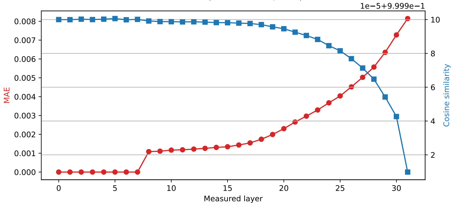
Mistral-7B-Instruct-v0.3 | Quantized layer 7 | float16 → int8
