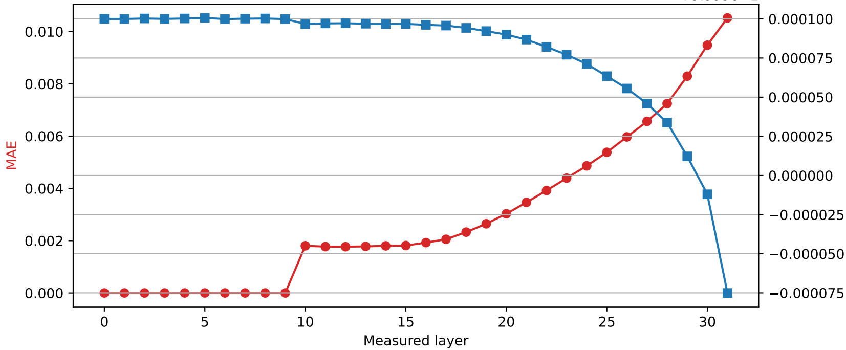
Mistral-7B-Instruct-v0.3 | Quantized layer 9 | float16 \rightarrow int8
