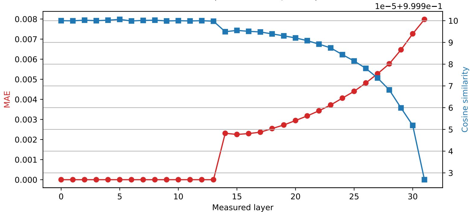
Mistral-7B-Instruct-v0.3 | Quantized layer 13 | float16 \rightarrow int8
