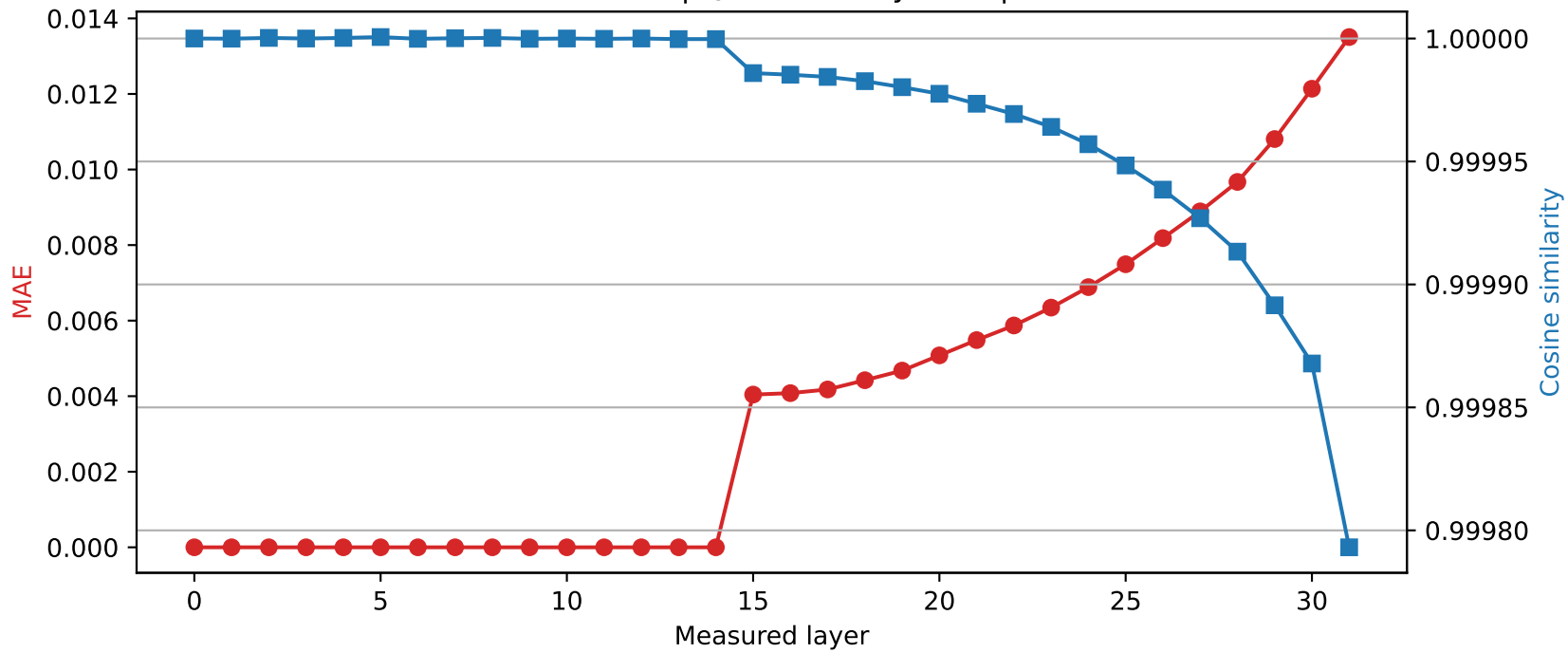
Mistral-7B-Instruct-v0.3 | Quantized layer 14 | float16 \rightarrow int8
