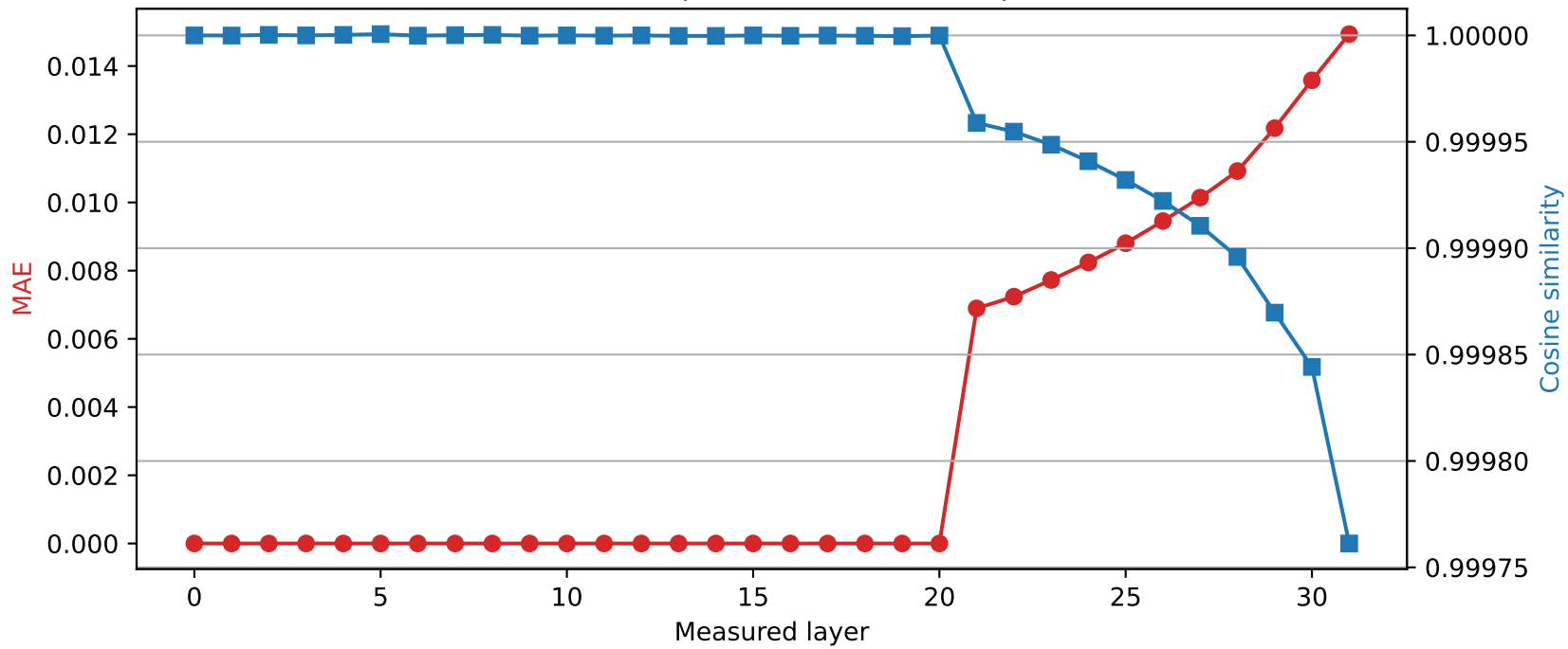
Mistral-7B-Instruct-v0.3 | Quantized layer 20 | float16 \rightarrow int8
