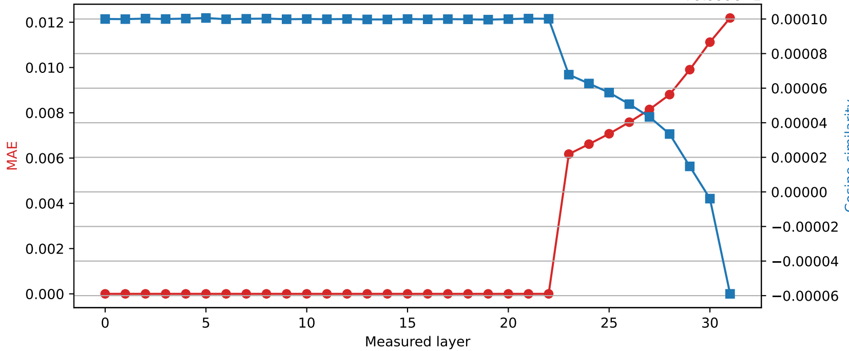
Mistral-7B-Instruct-v0.3 | Quantized layer 22 | float16 \rightarrow int8 +9.999e-1
