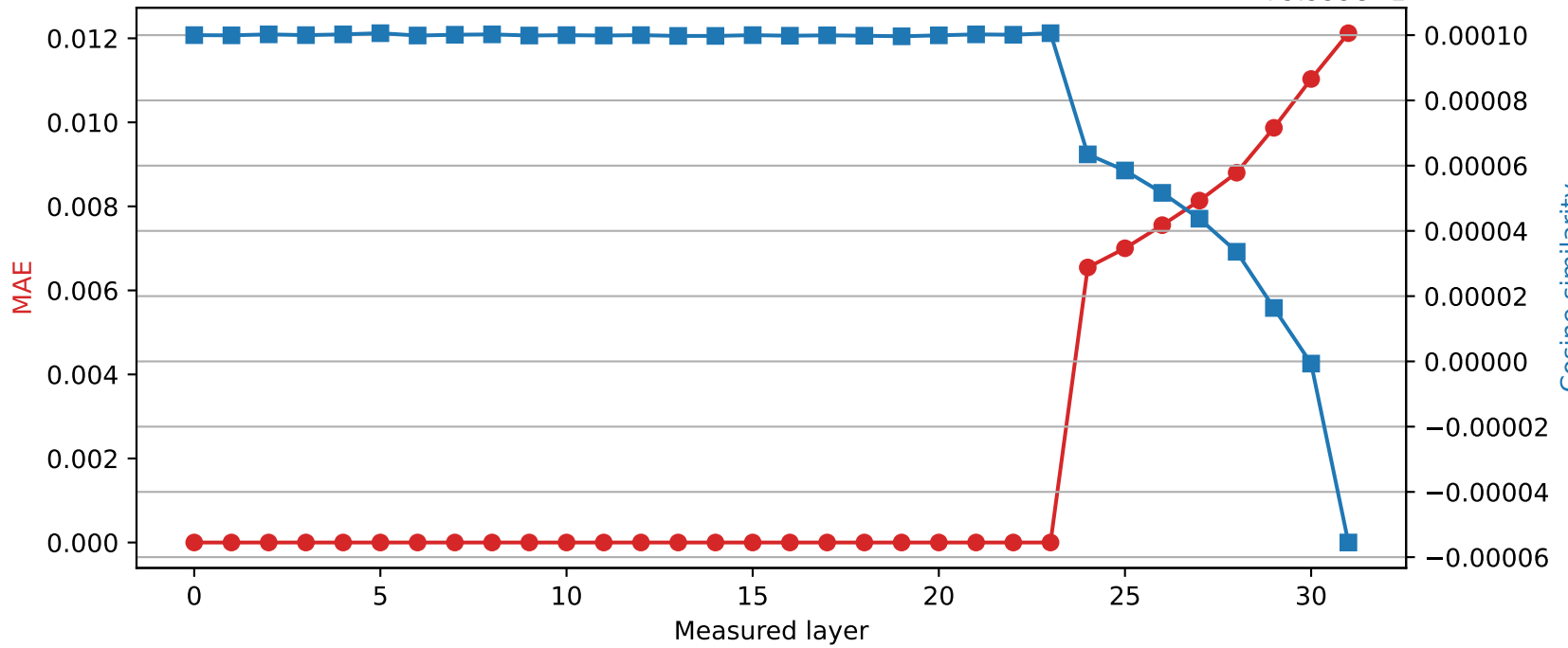
Mistral-7B-Instruct-v0.3 | Quantized layer 23 | float16 \rightarrow int8 +9.999e-1
