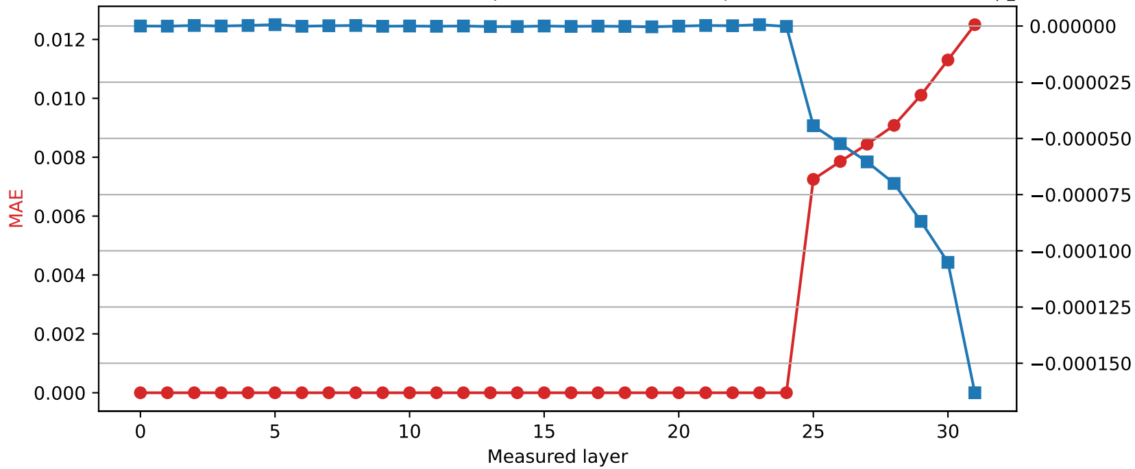
Mistral-7B-Instruct-v0.3 | Quantized layer 24 | float16 → int8
